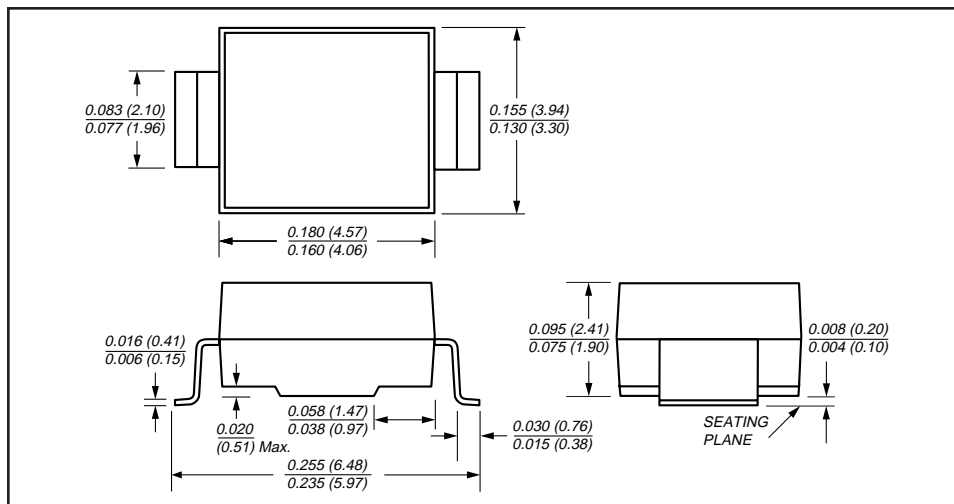
DO-215AA (SMBG GULL WING)
