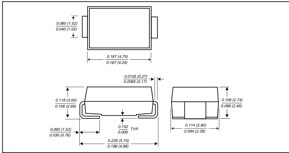
DO-214BA (GF1)
