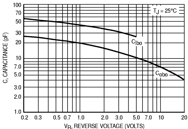
Figure 7. Capacitances
