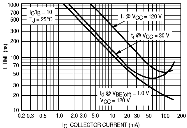
Figure 8. Turn-On Time
