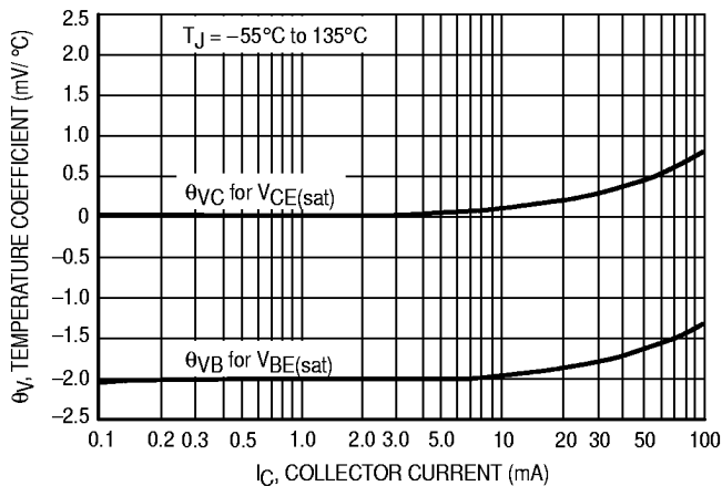
Figure 5. Temperature Coefficients
