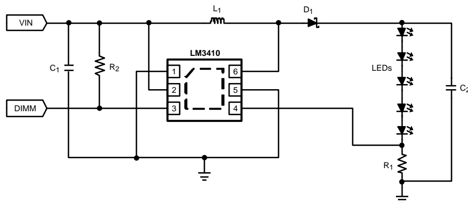
Figure 1. LM3410X 6-Pin LLP Schematic
