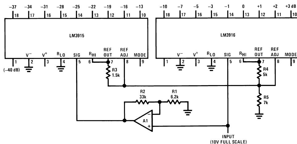
Figure 12. Improved Circuit for 40 dB Display
