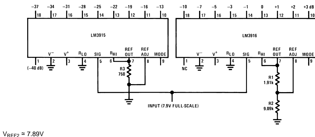
Figure 11. Low Cost Circuit for 40 dB Display
