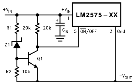
Figure 17. Undervoltage Lockout for Buck Circuit
