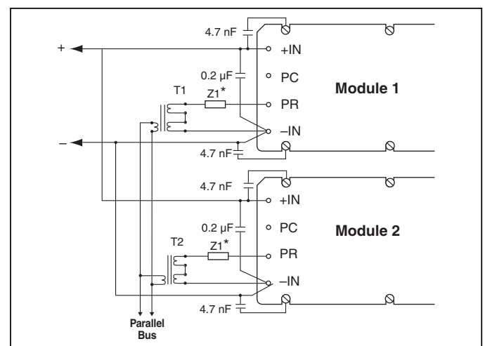
Figure 10 — Transformer-coupled interface.
