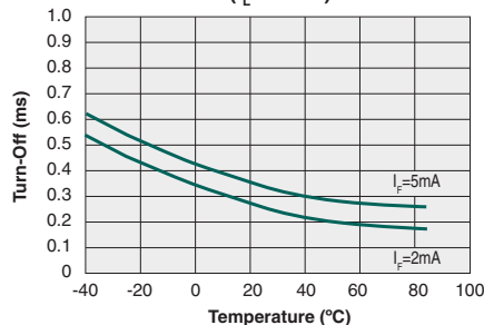
Typical Turn-Off vs. Temperature ( I_L=50\text{mA} )
