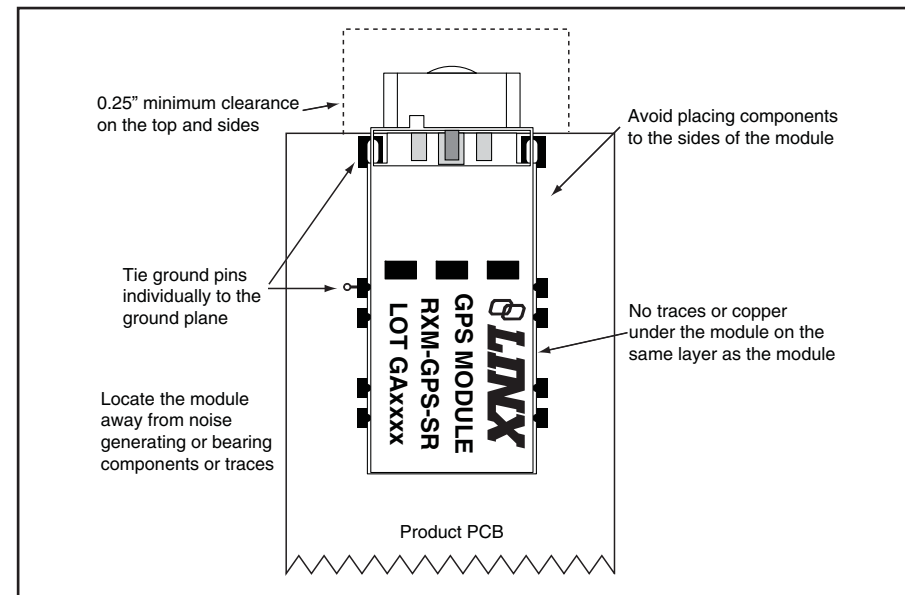
Figure 6: Antenna Considerations
