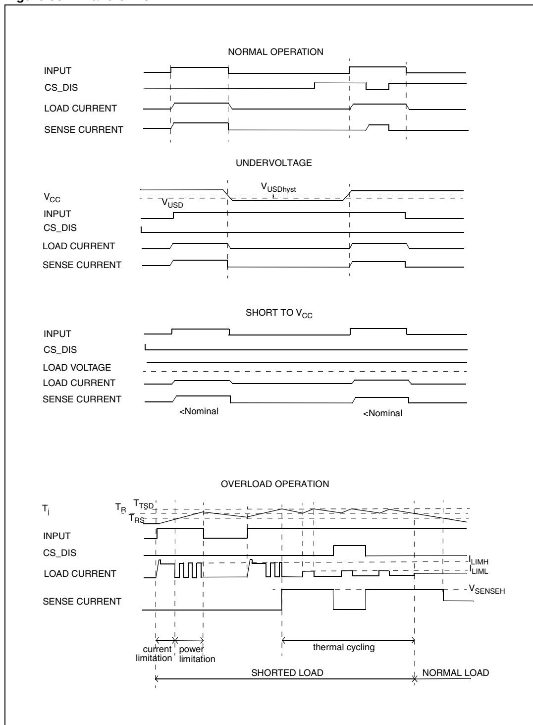
Figure 35. Waveforms
