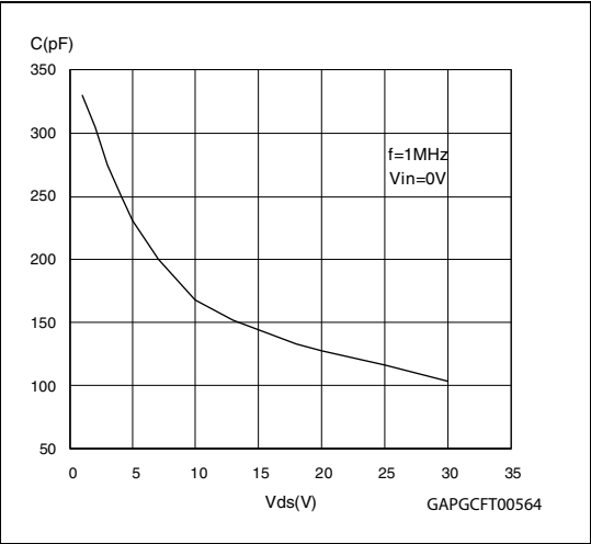
Figure 23. Capacitance variations
