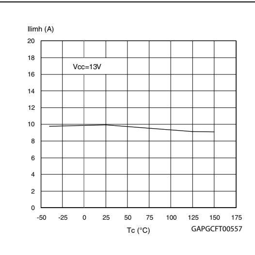
Figure 16. I_{LIMH} vs T_{case}
