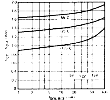
Figure 8. High Output Voltage
