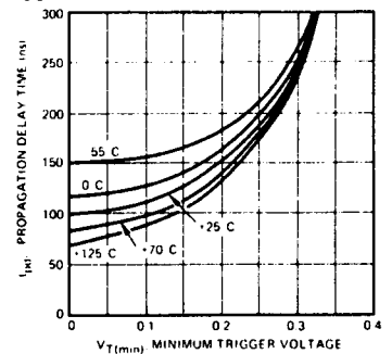
Figure 14. Propagation Delay vs. Trigger Voltage
