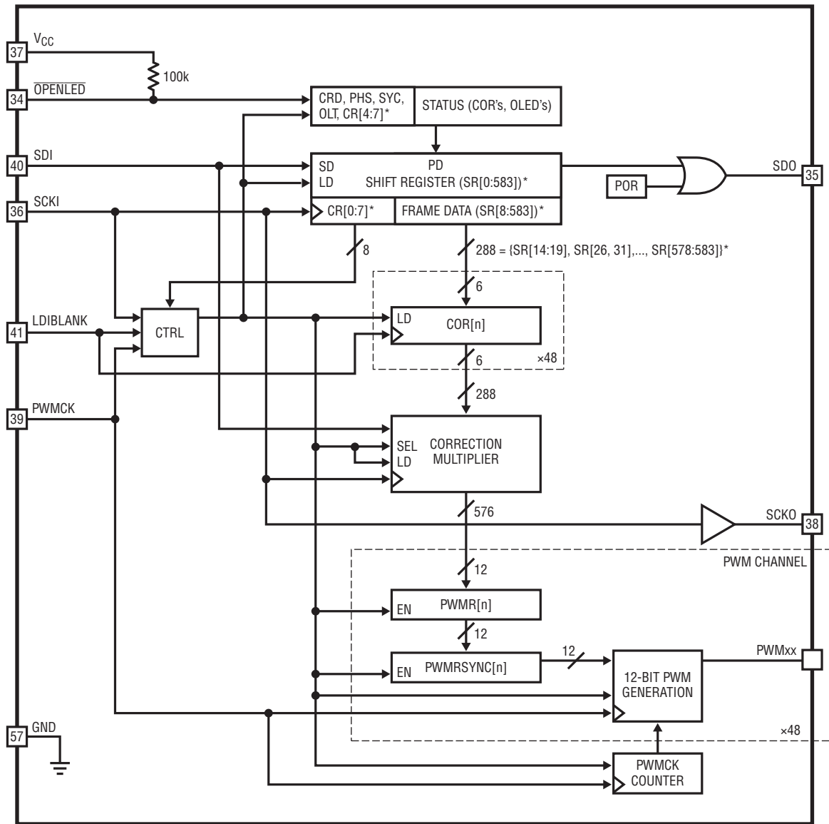
Figure 1. Block Diagram
