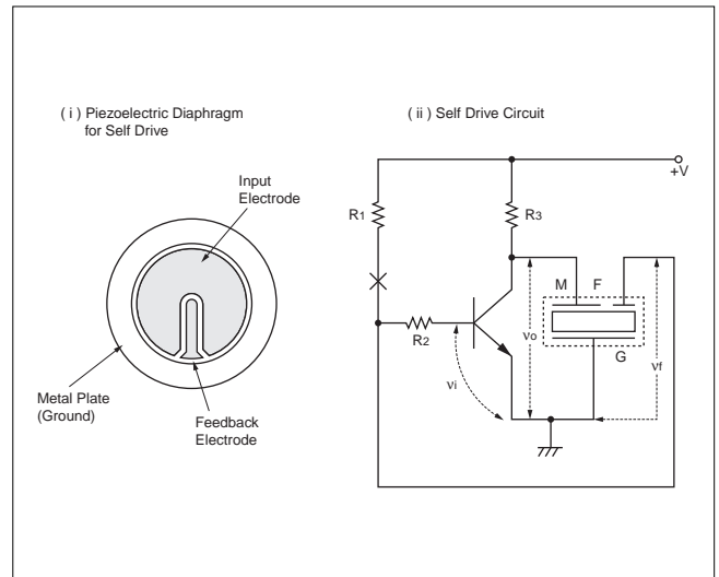
Fig. 9 Self Drive Circuit
