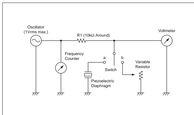
Fig. 13 Measurement Set Up of Resonant Freq. and Resonant Impedance
