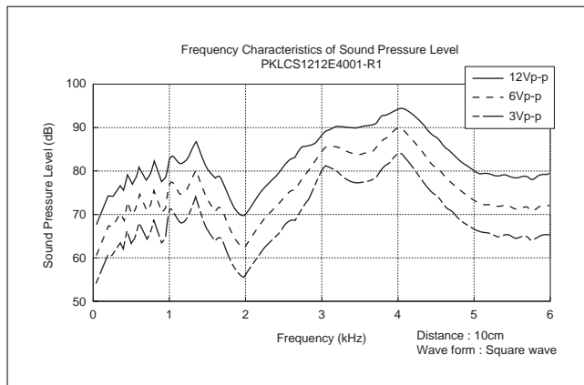
Fig. 10 Frequency Characteristics of Sound Pressure Level
