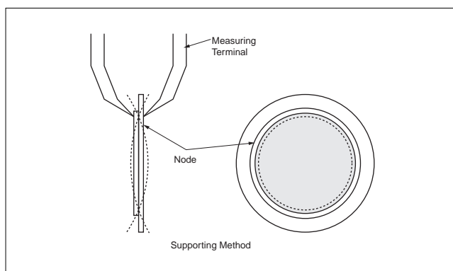
Fig. 12 Measurement of Piezoelectric Diaphragm
