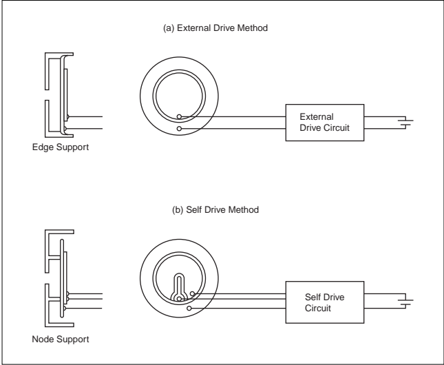
Fig. 5 Drive Procedures
