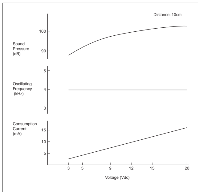
Fig. 15 Voltage Characteristics
