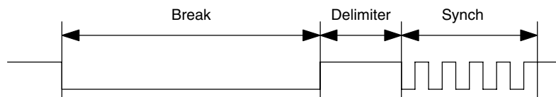
Figure 19–5. Auto Baud Rate Detection – Break/Synch Sequence
