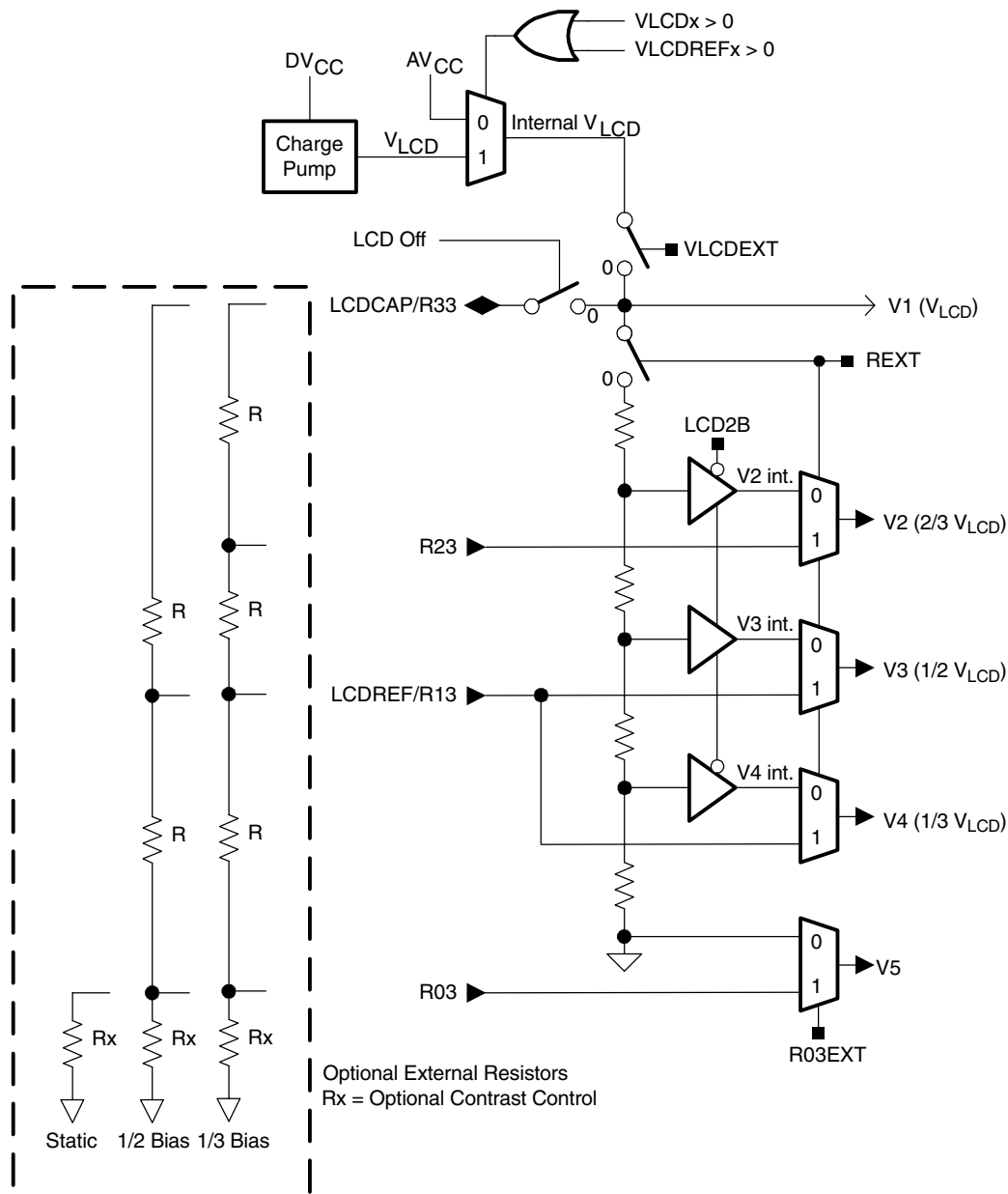
Figure 26–3. Bias Generation
