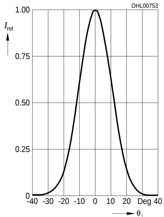
Far-field distribution perpendicular to junction I_{\text{rel}} vs. \theta_{\parallel} ( T_A = 25^\circ\text{C} , P_{\text{opt}} = 4\text{ W} )
