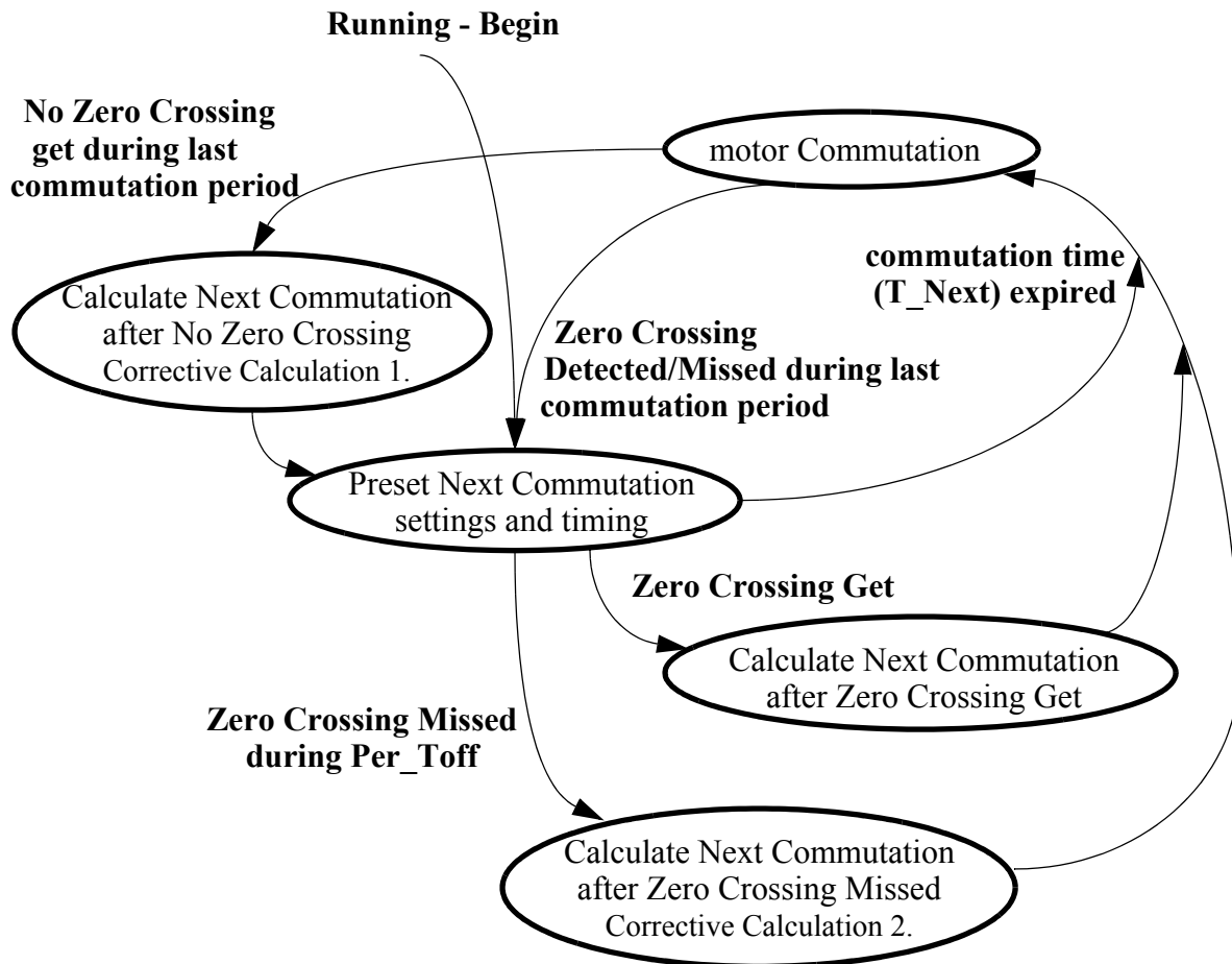
Figure 7-9. Substates - Running
