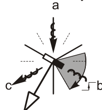
Figure 5-9. Vectors of Magnetic Fields
