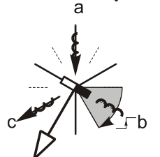
Figure 5-9. Vectors of Magnetic Fields
