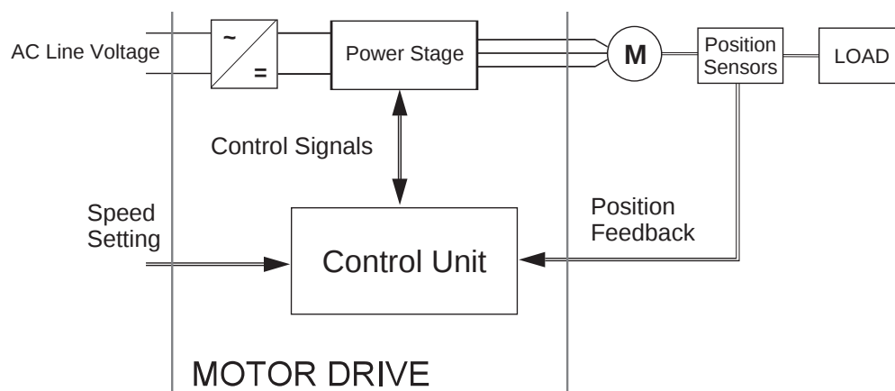
Figure 3-4. Classical System
