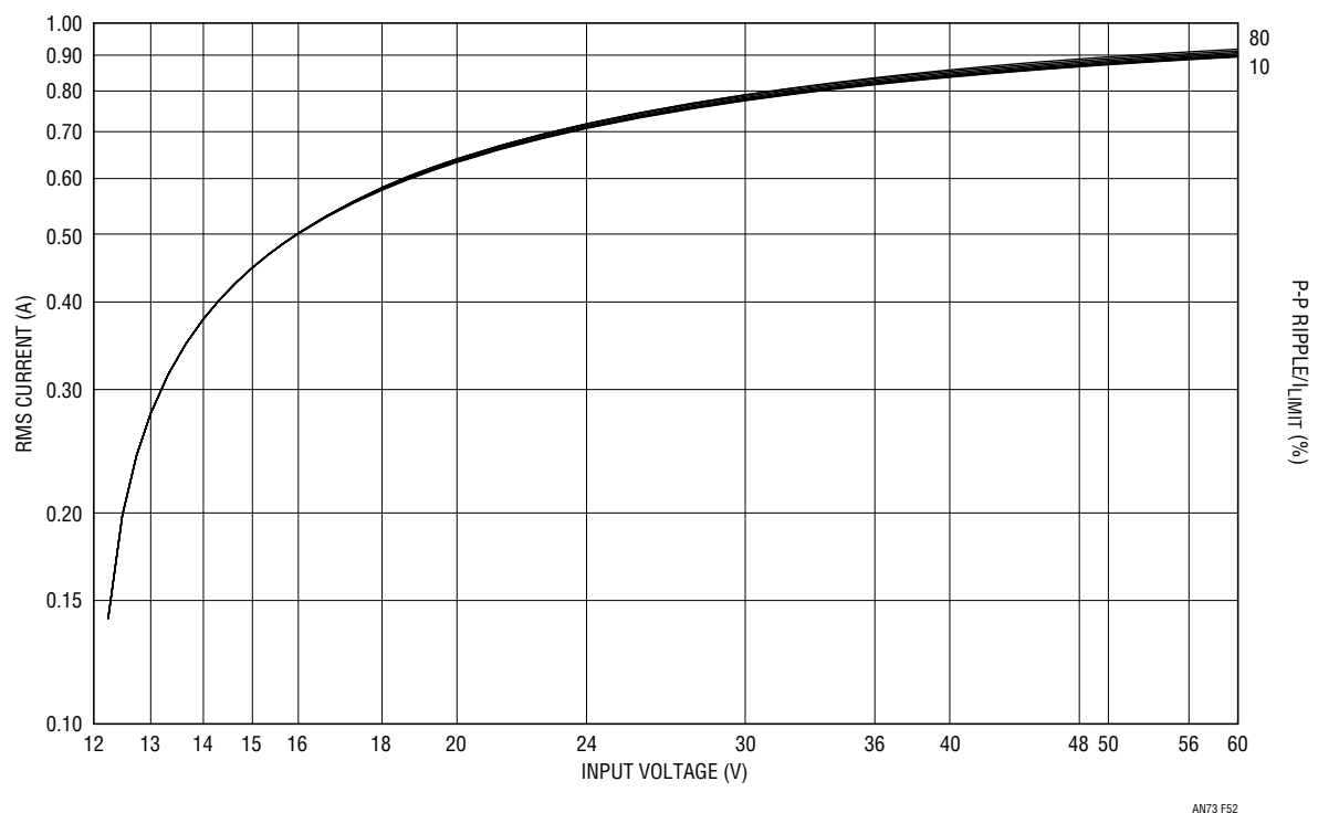
Figure 52. 12V Output Normalized RMS Bottom Transistor Current
