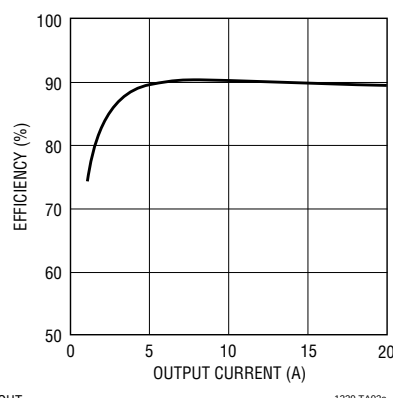
28V to 5V Efficiency
