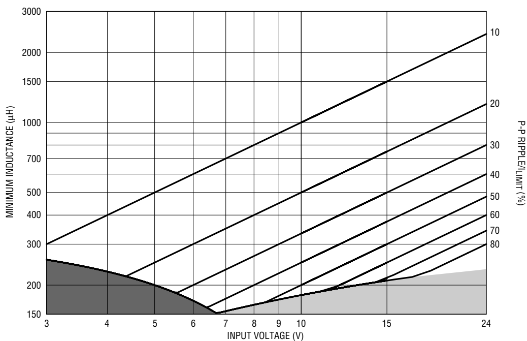
Figure 62. 24V Output Normalized Minimum Inductor Value
