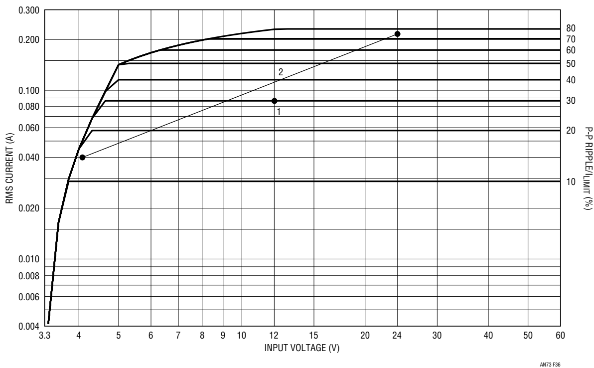
Figure 36. 3.3V Output Normalized Output Capacitor AC RMS Current
