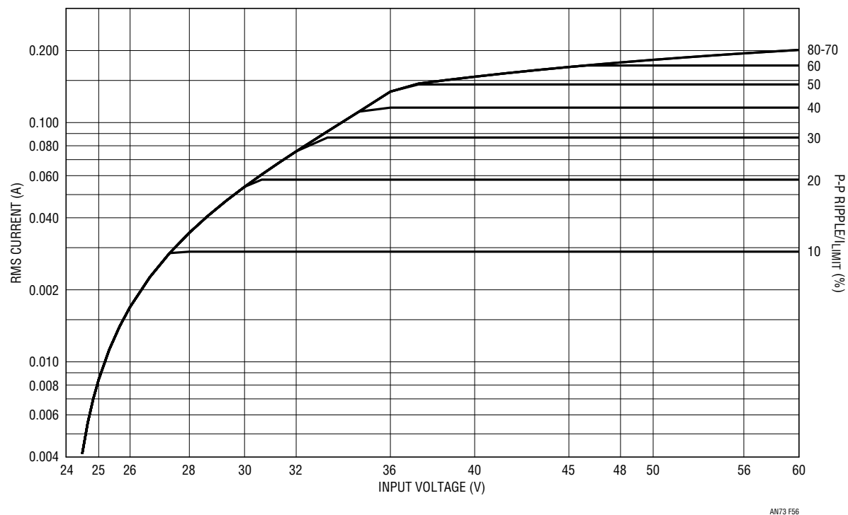
Figure 56. 24V Output Normalized Output Capacitor AC RMS Current
