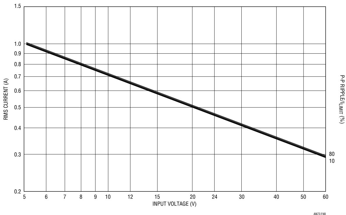
Figure 48. 5V Output Normalized Top Switch RMS Current
