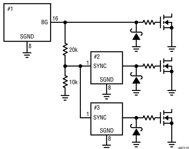
Figure 5. Master/Slave Synchronization
