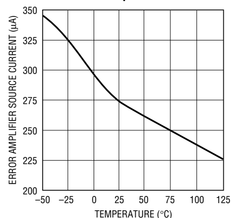
Error Amplifier Maximum Source Current vs Temperature
