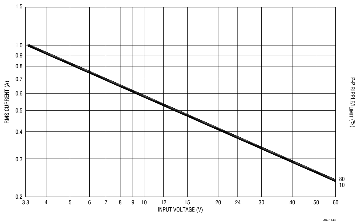
Figure 43. 3.3V Output Normalized Top Switch RMS Current
