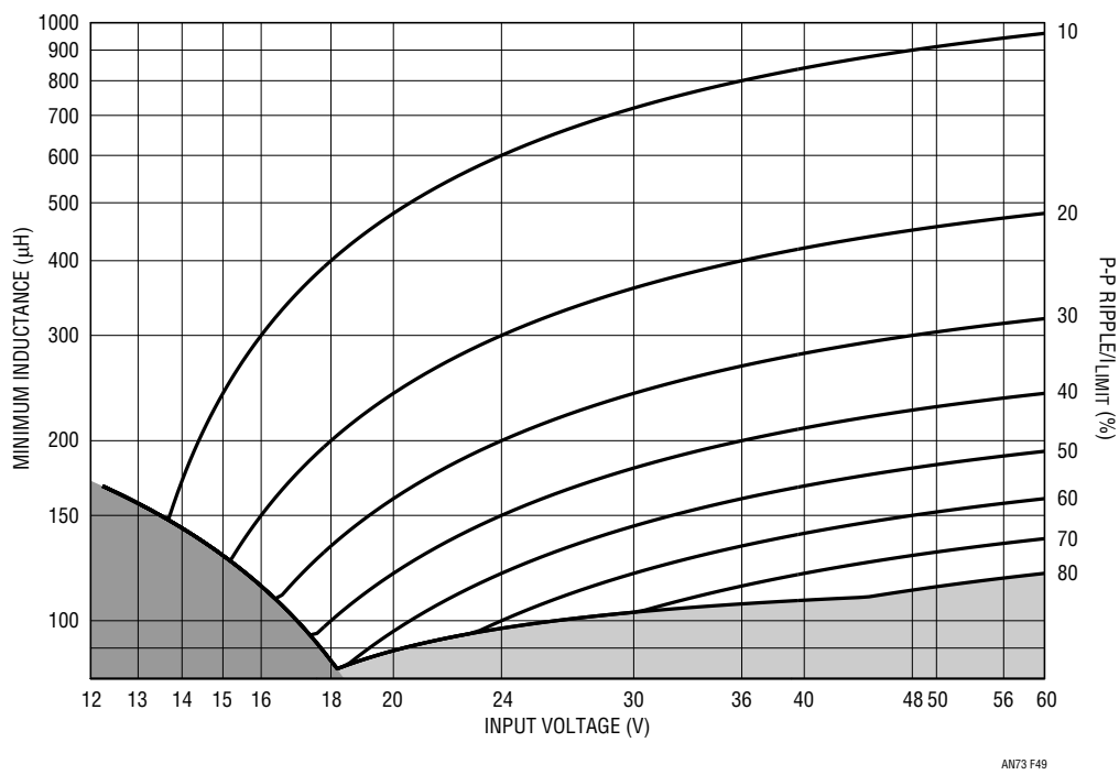
Figure 49. 12V Output Normalized Minimum Inductor Value
