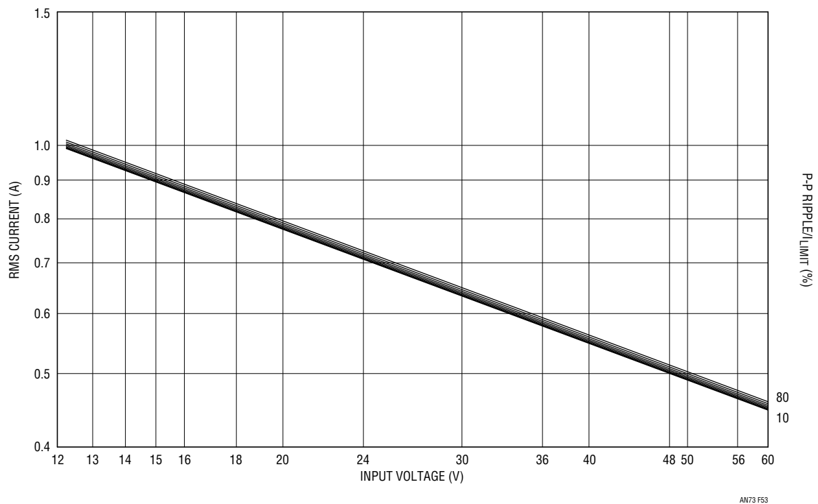
Figure 53. 12V Output Normalized Top Switch RMS Current
