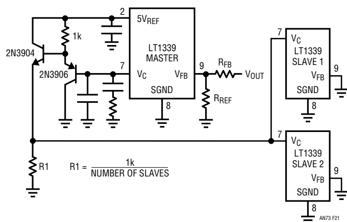
Figure 21. Master/Slave Current Sharing
