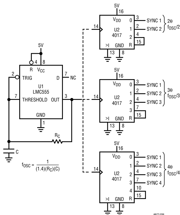
Figure 6. Multiphase Synchronization
