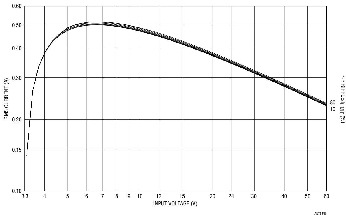
Figure 40. 3.3V Output Normalized RMS AC Input Capacitor Current
