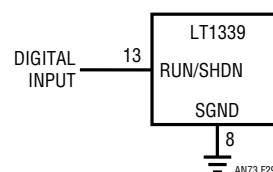
Figure 29c Digital Shutdown
