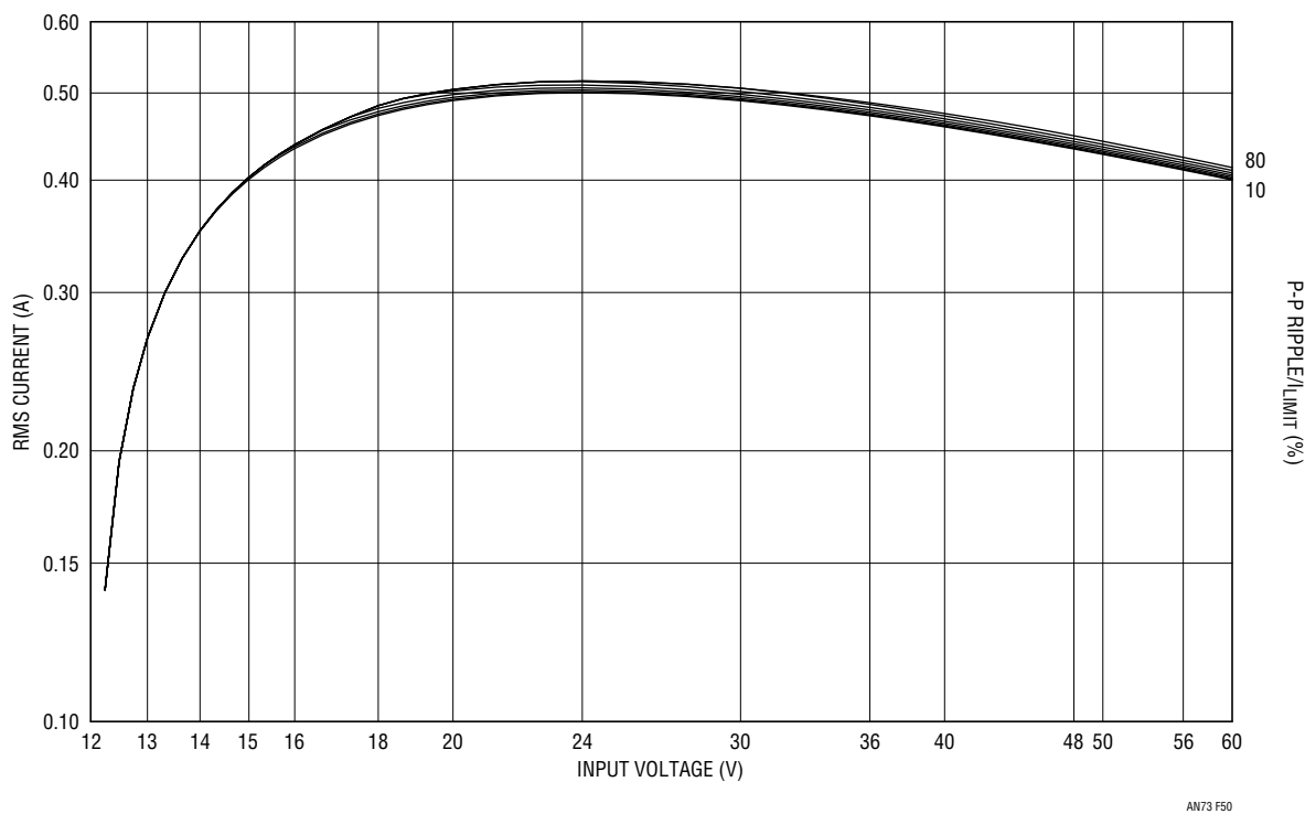
Figure 50. 12V Output Normalized RMS AC Input Capacitor Current
