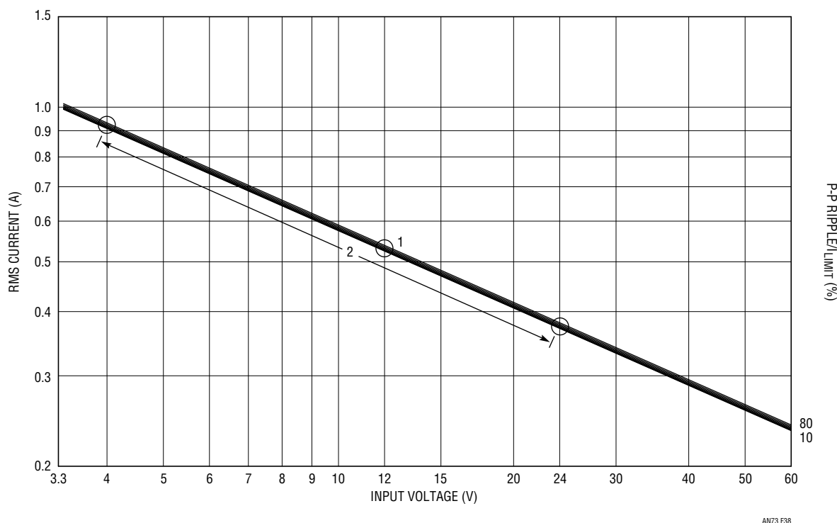
Figure 38. 3.3V Output Normalized Top Switch RMS Current
