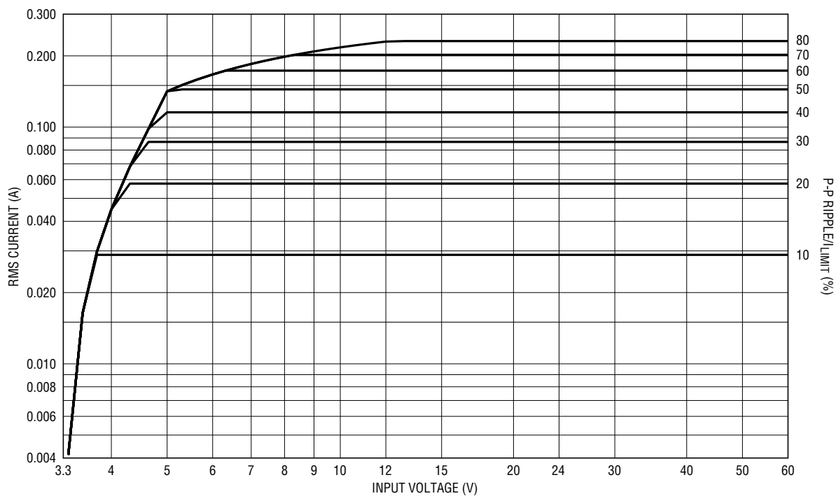
Figure 41. 3.3V Output Normalized Output Capacitor AC RMS Current
