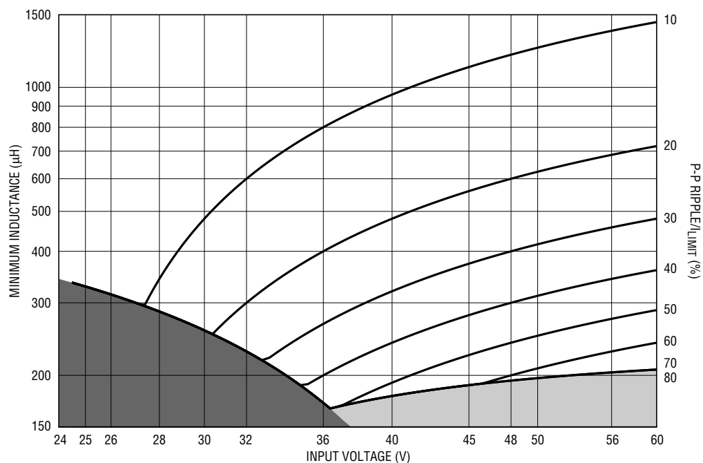
Figure 54. 24V Output Normalized Minimum Inductor Value
