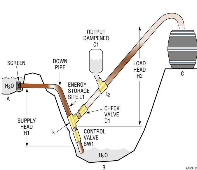
Figure 1. Hydraulic Impulse Pump (Water Hammer)
