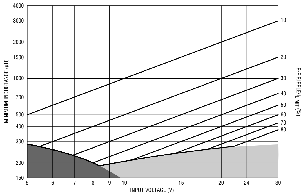
Figure 63. 30V Output Normalized Minimum Inductor Value
