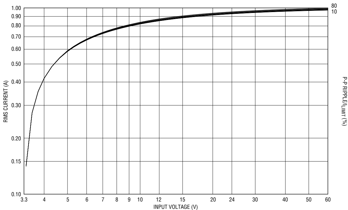
Figure 42. 3.3V Output Normalized RMS Bottom Transistor Current
