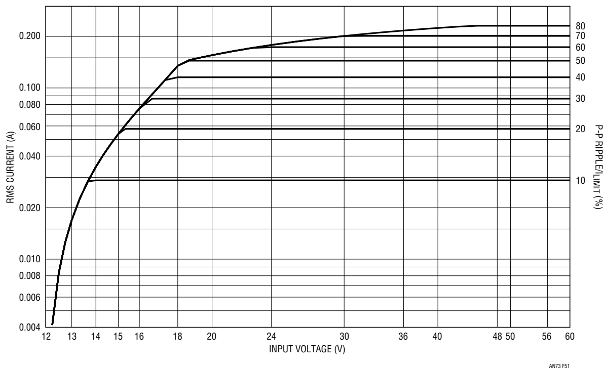
Figure 51. 12V Output Normalized Output Capacitor AC RMS Current
