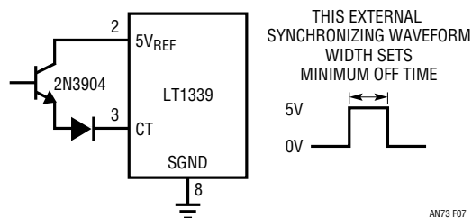
Figure 7. Wide-Range Synchronization Using the CT Pin
