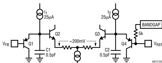
Figure 25. Error Amplifier Input Stage
