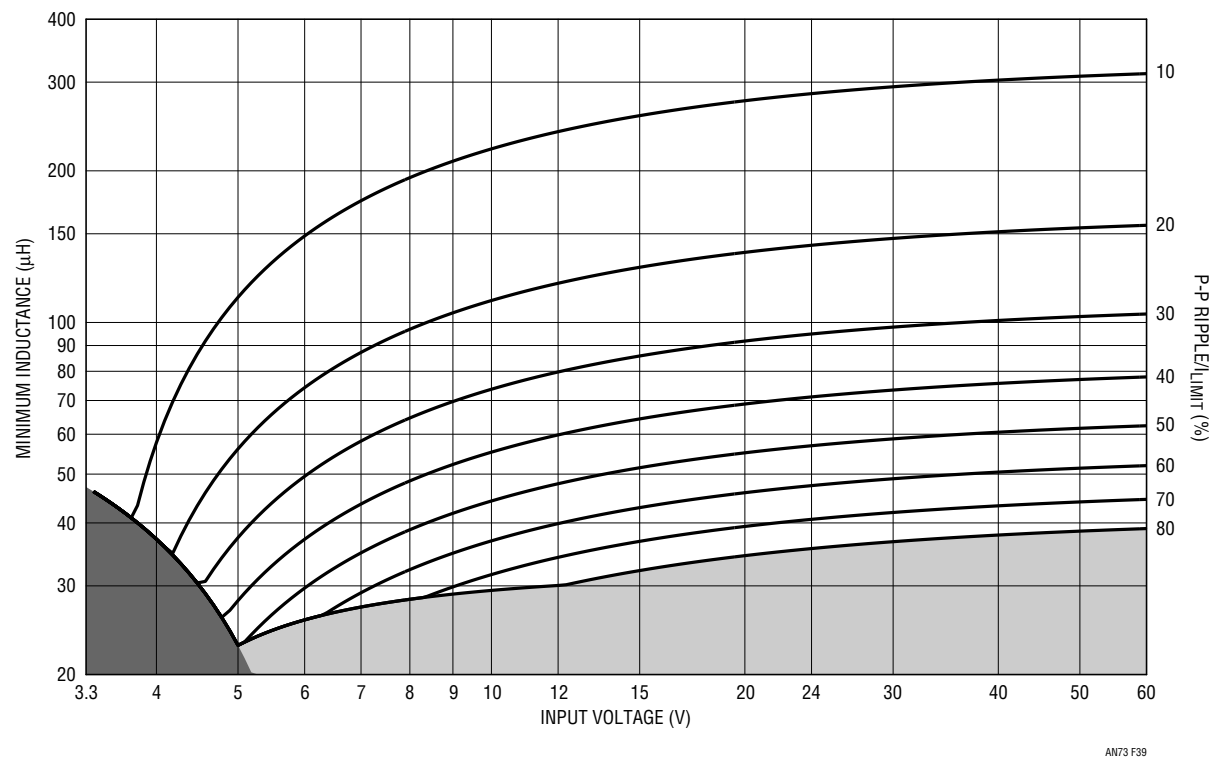
Figure 39. 3.3V Output Normalized Minimum Inductor Value
