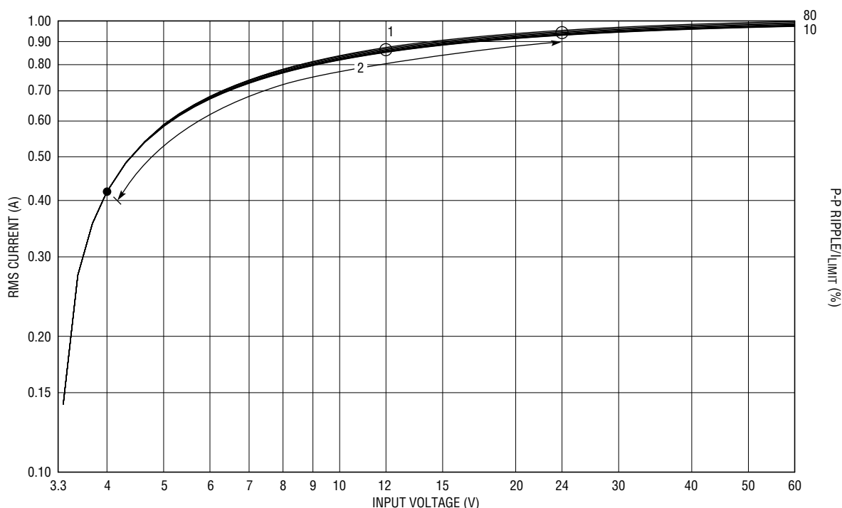
Figure 37. 3.3V Output Normalized RMS Bottom Transistor Current
