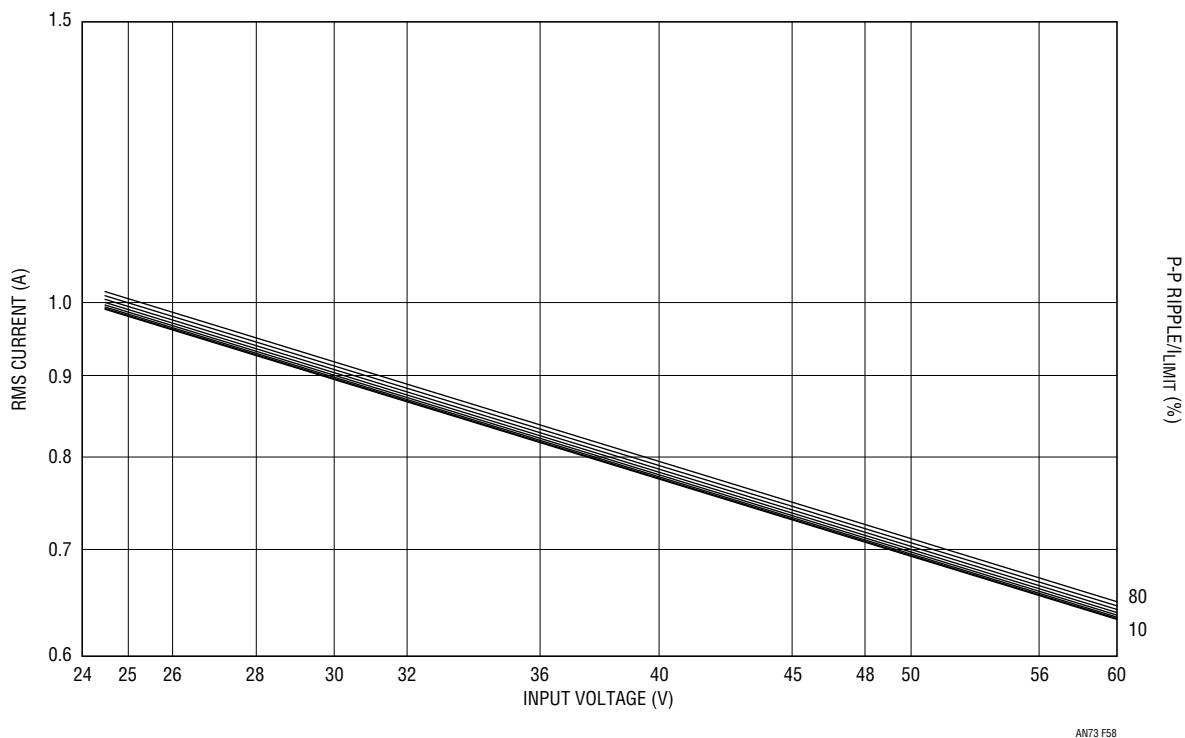
Figure 58. 24V Output Normalized Top Switch RMS Current
