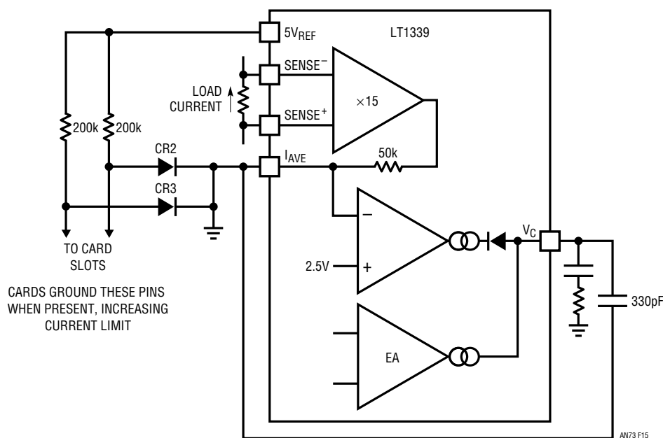
Figure 15. Multiple Level Automatic Current Limit
