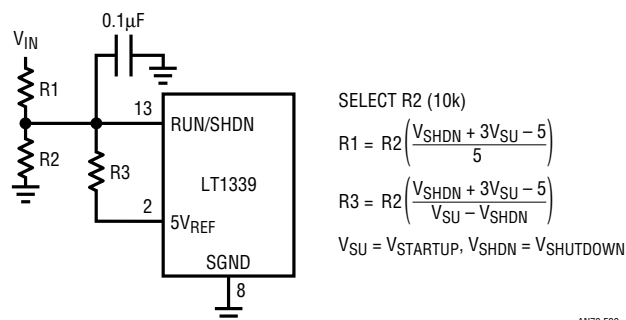
Figure 29a RUN/SHDN Pin
