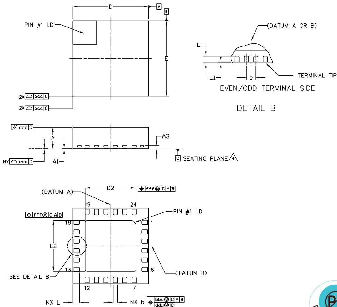
Figure 25. TQFN(4x4)-24 Package
