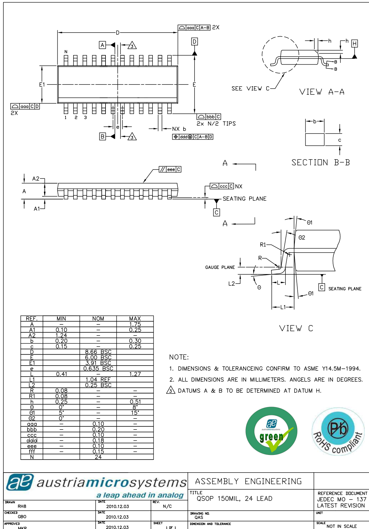
Figure 24. QSOP-24 Package
