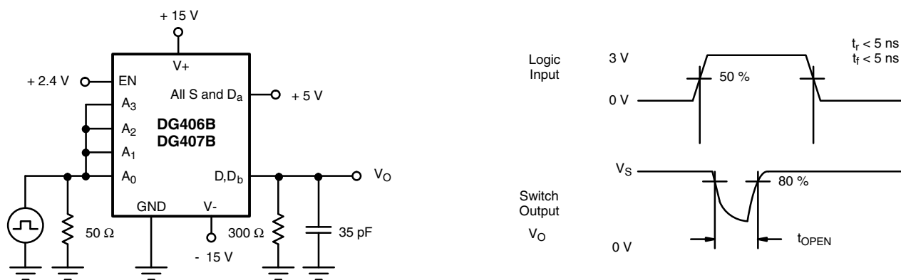
Figure 4. Break-Before-Make Interval
