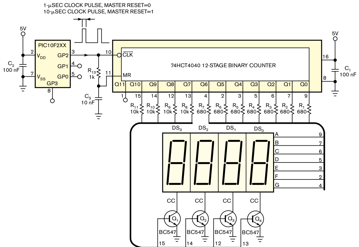
Figure 3 The same technique works with seven-segment displays.
