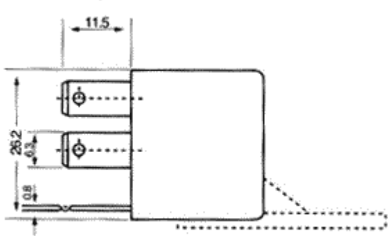
1 Form A
