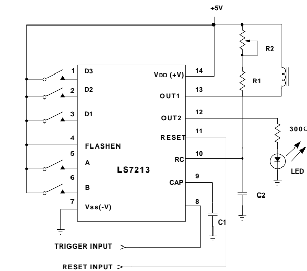
FIGURE 4. TYPICAL APPLICATION WITH OUT1 AS RELAY DRIVE AND OUT2 AS FLASHER
