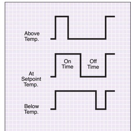
Figure 1: Proportional control
