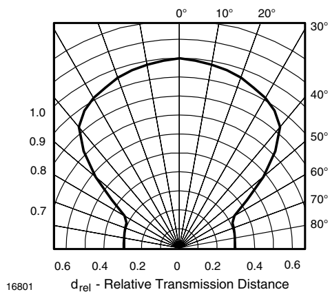
Fig. 10 - Horizontal Directivity
