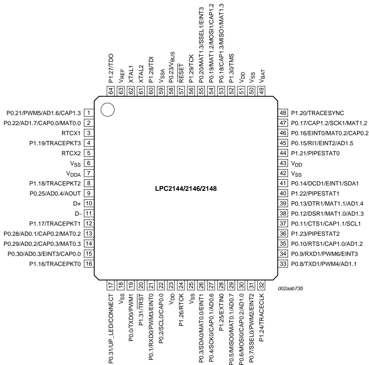
Fig 15. LPC2144/6/8 64-pin package
