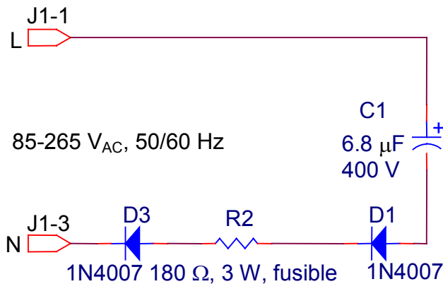
Figure 8.6.1 - Configuration “1”, 2 kV.
