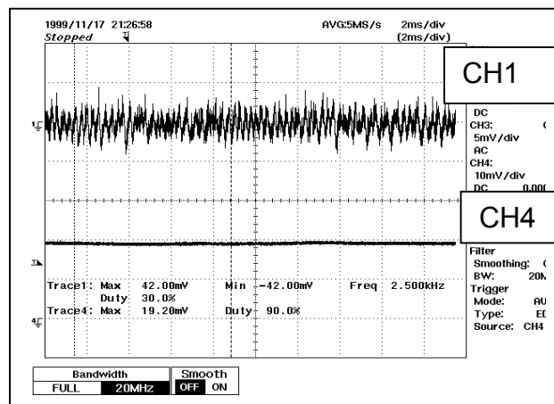
Figure 8.4.3.2 - Switching Frequency Ripple at Full Load. CH1: V_{OUT} (50 mV/div), CH4: I_{OUT} (50 mA/div)
