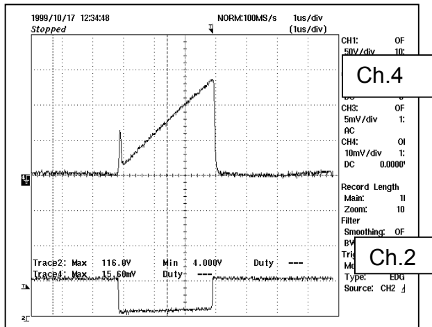
Figure 8.4.2.1 - Full Load at 85 V AC .
