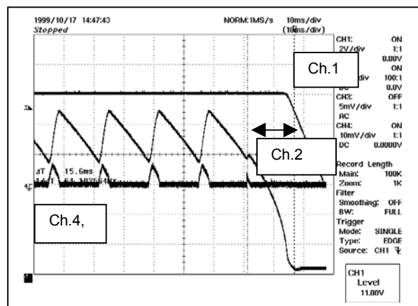
Figure 8.4.1.2 - Output Voltage Hold Up Time.
