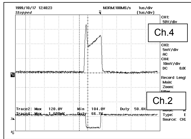
Figure 8.4.2.2 - Short Circuit at 85 V AC .
