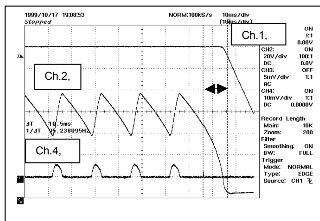
Figure 8.4.1.4 - Output Voltage Hold-up Time at Full Load.
