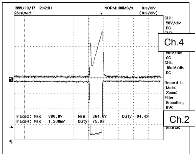
Figure 8.4.2.3 - Full Load at 265 V AC .
