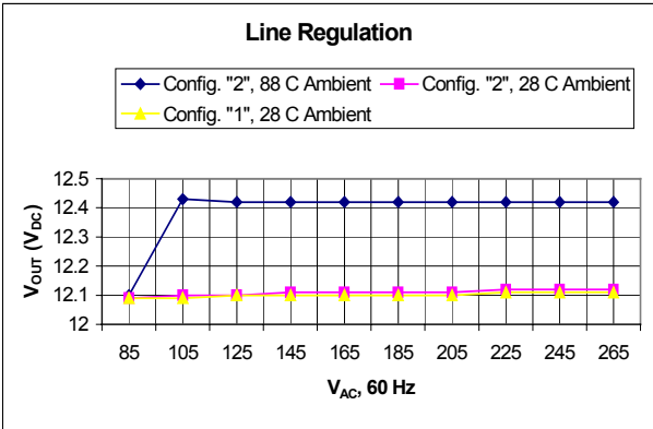
Figure 5.2.1 – Line Regulation at Full Load, 28 °C Ambient.
