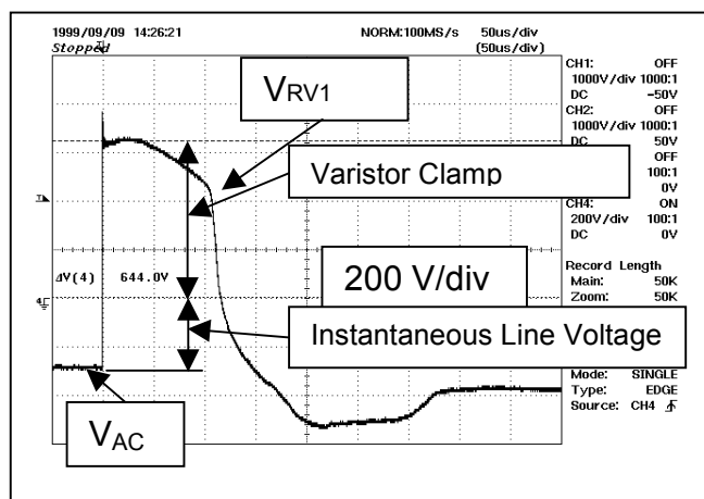
Figure 8.6.3 - RV1 Voltage During +6 kV, 1.2/50 \mu s Surge.
