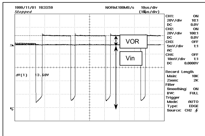
Figure 8.4.2.5 - Drain-Source Voltage ( V_{DS} ). CH2 (20 V/div). V_{OR}=V_O+V_D=13.6 V
