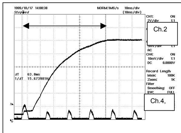
Figure 8.4.1.1 - Output Voltage Turn On Delay at Full Load.
