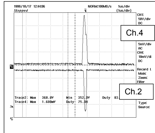
Figure 8.4.2.4 - Short Circuit at 265 V AC .
