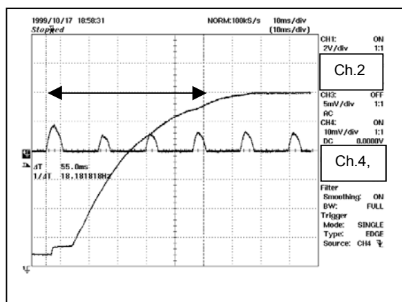
Figure 8.4.1.3 - Output Voltage Turn-on Delay at Full Load.
