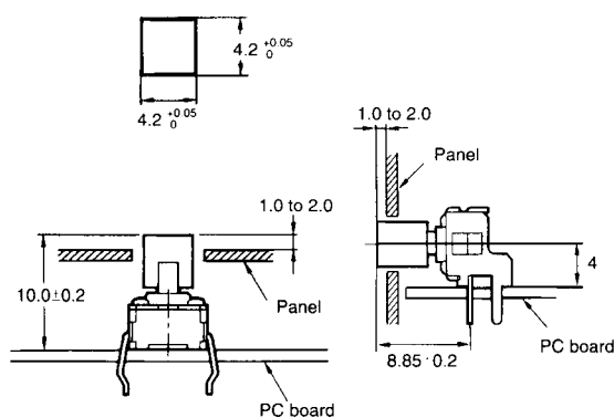
Panel Cutout
