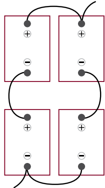
To increase both voltage and amp-hour capacity, connect batteries in series/parallel.
