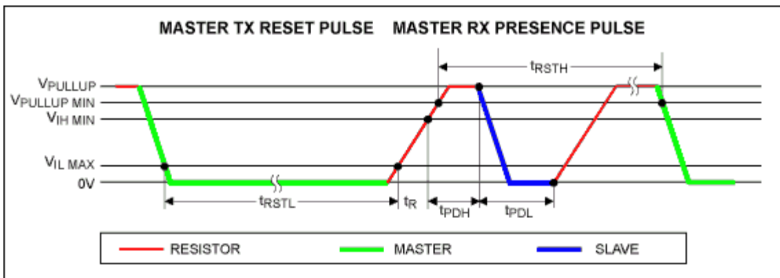
Figure 4. Legacy reset and presence pulse.
