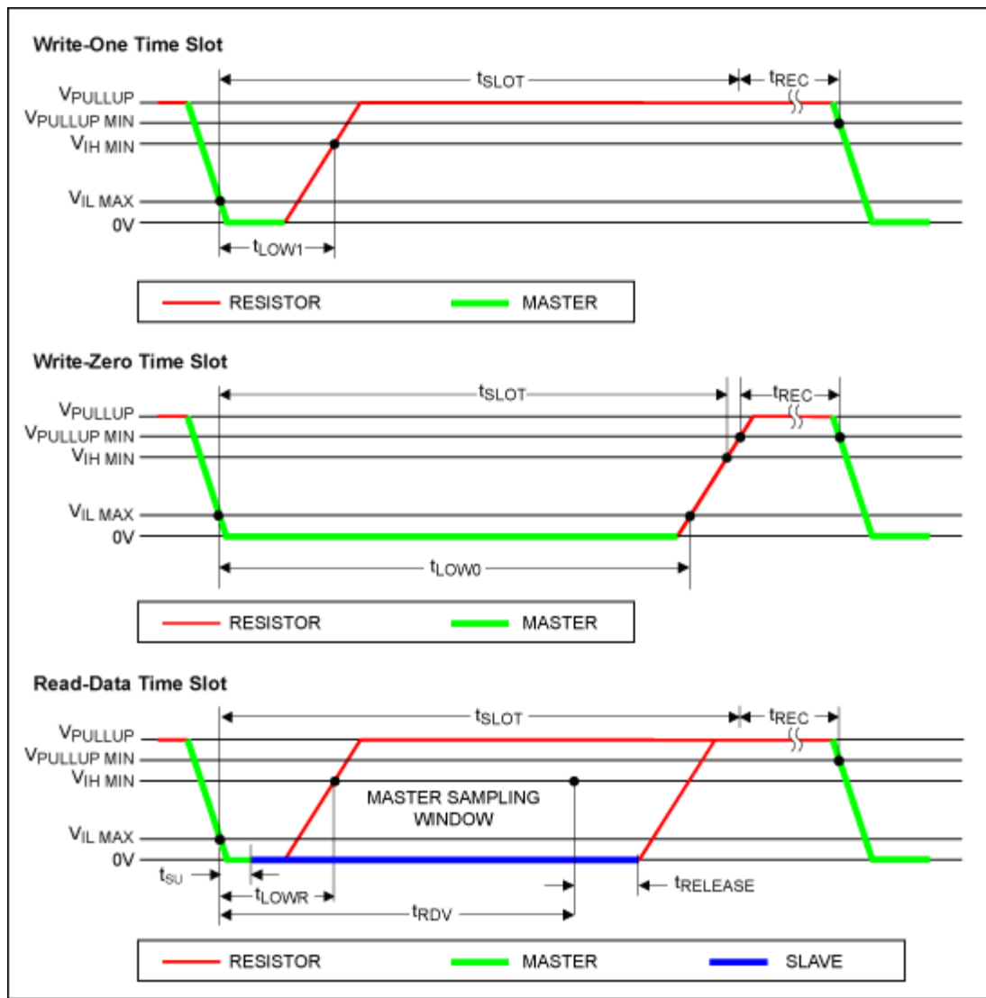
Figure 5. Legacy read/write timing diagram.
