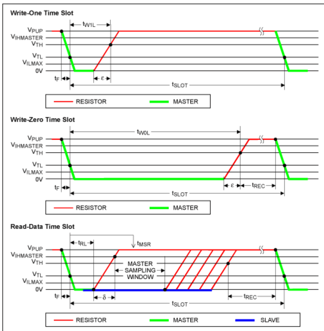
Figure 2. Read/write timing diagram.
