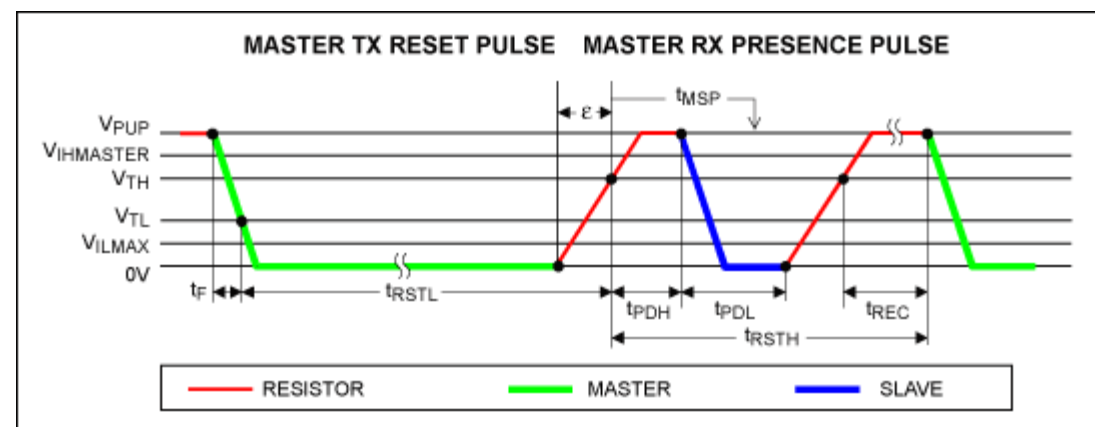
Figure 1. Reset and presence pulse.
