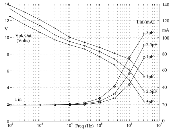
Figure 11: Peak driver output voltage and input supply current for different loads plotted against frequency.
