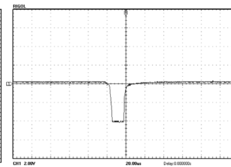
Waveform of Signal-L and Signal-R (CH1 2V 20.00us)
