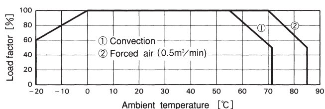
Fig.5.2 Derating curve
