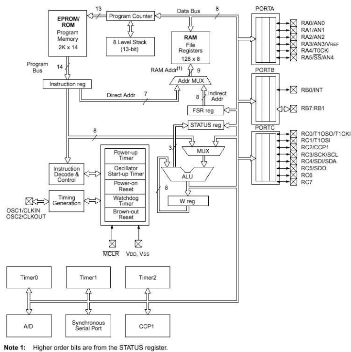
Figure 1: Block diagram of a PIC microcontroller
