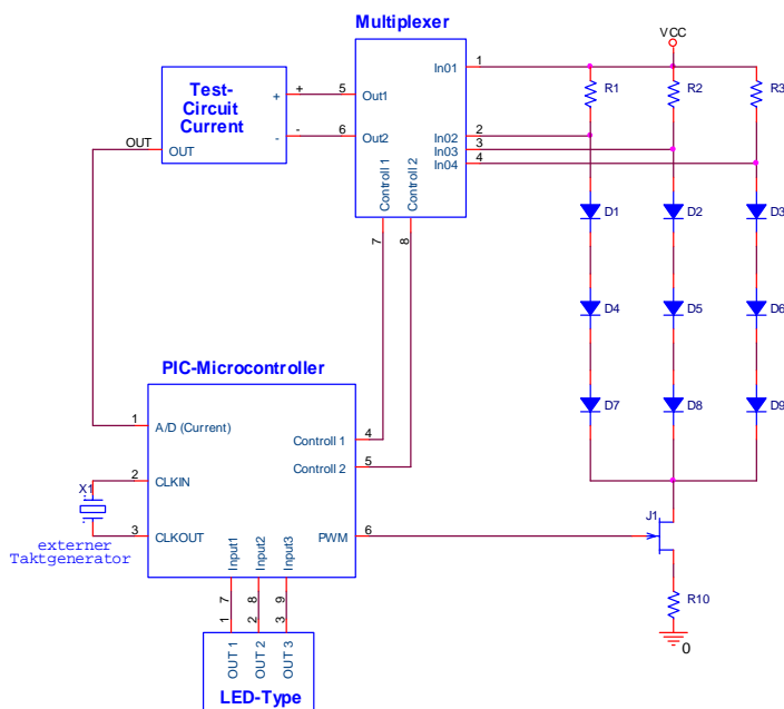
Figure 9: Circuit example with serial connection
