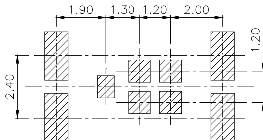
Figure A.18.2(a) M4-outline substrate/PCB layout
