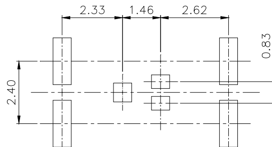
Figure A.16.3(a) MU-outline stencil design
