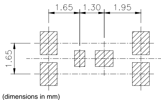
Figure A.2.2(a) SQ-outline substrate/PCB layout
