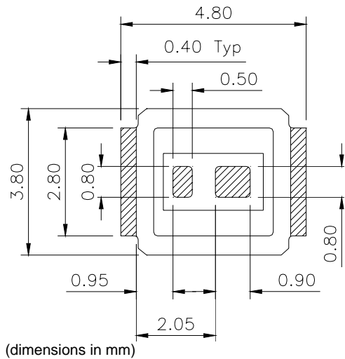
Figure A.2.1 SQ-outline device outline
