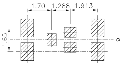
Figure A.9.2(a) SC-outline substrate/PCB layout
