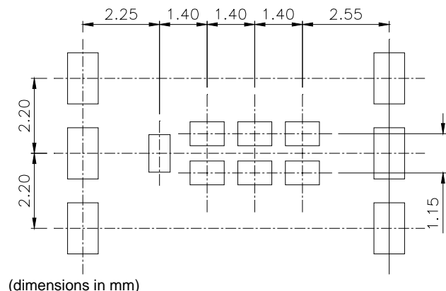
Figure A.20.3(a) L6-outline stencil design
