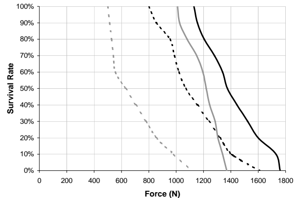
— 6601 Continuous - - 6601 Stepped — 6602 Continuous - - 6602 Stepped Figure 22 DirectFET survival rates
