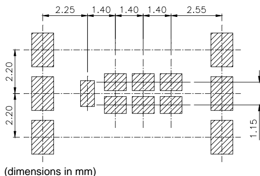
Figure A.20.2(a) L6-outline substrate/PCB layout
