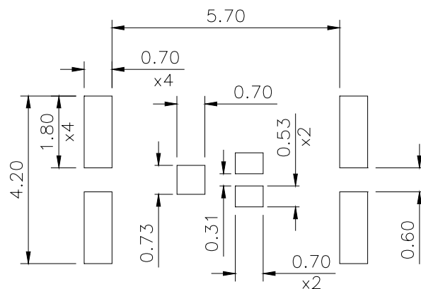
Figure A.16.3(b) MU-outline stencil design
