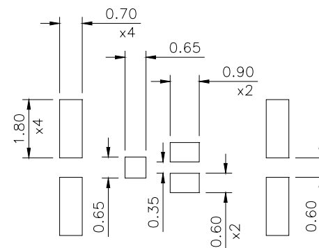
Figure A.15.3(a) MZ-outline stencil design
