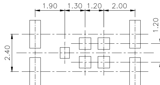
Figure A.18.3(a) M4-outline stencil design
