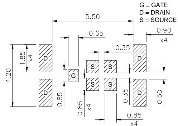
Figure A.18.2(b) M4-outline substrate/PCB layout
