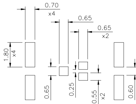
Figure A.13.3(a) MQ-outline stencil design
