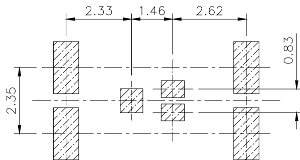
Figure A.16.2(a) MU-outline substrate/PCB layout
