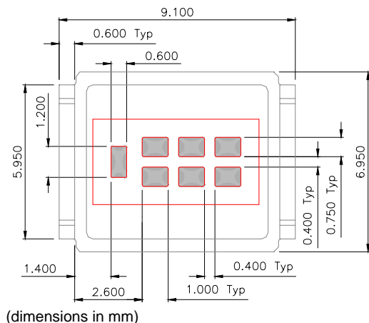
Figure A.20.1 L6-outline device outline
