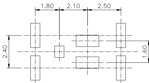
Figure A.10.3(a) MT-outline stencil design
