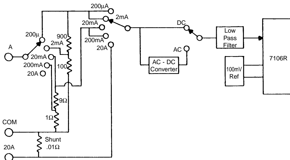
Figure 4 Simplified Current Measurement Diagram
