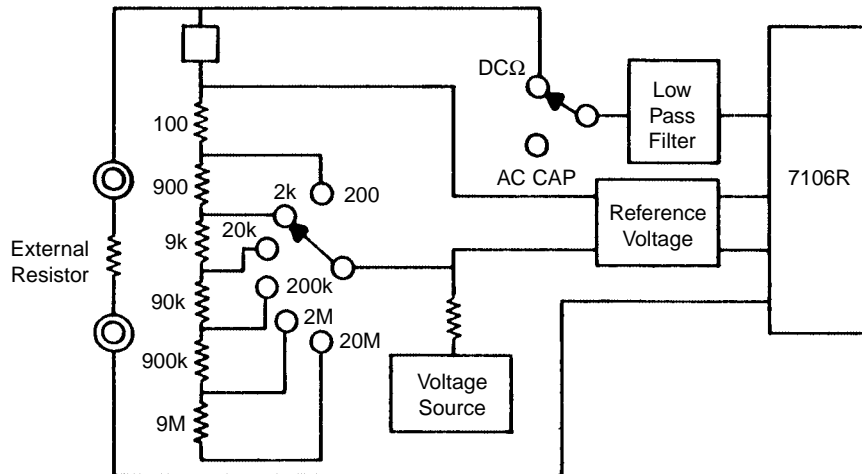
Figure 5 Simplified Resistance Measurement Diagram
