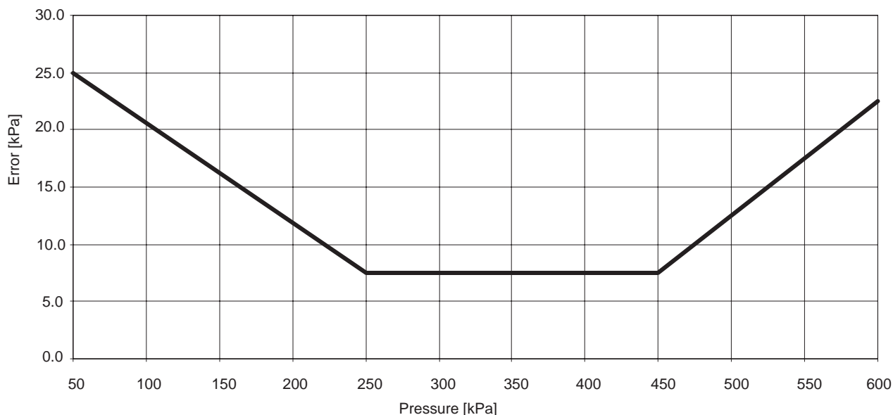
Figure 9. Pressure Error vs Pressure at T= 25°C, 2.7 \leq V_{DD} \leq +3.3 V
