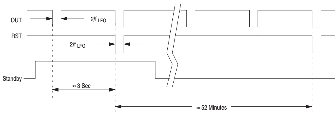
Figure 5. Pulse on \overline{\text{RST}} Pin
