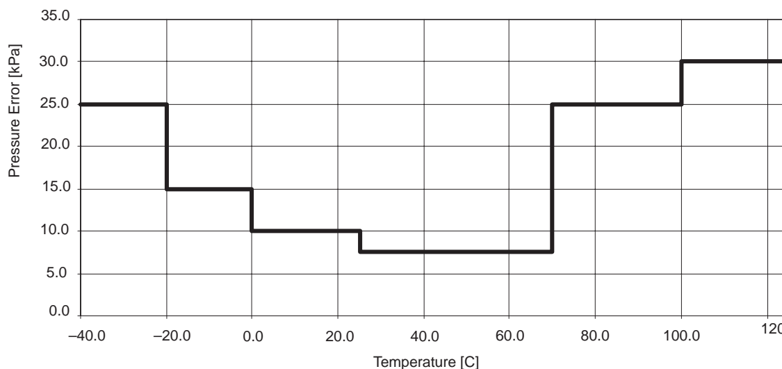
Figure 11. Pressure Error vs. Temperature at V_{DD} = 3 V, 250 \text{ kPa} \leq P \leq 450 \text{ kPa}
