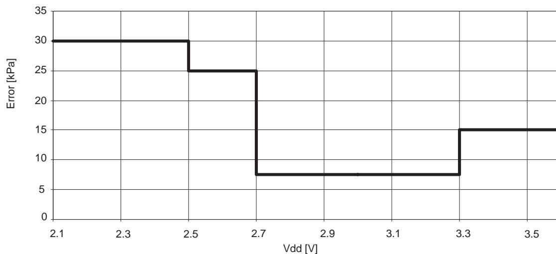
Figure 10. Pressure Error vs V_{DD} at 25°C, 250 \text{ kPa} \leq P \leq 450 \text{ kPa}
