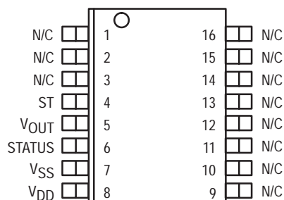
16-Pin SOIC Package
